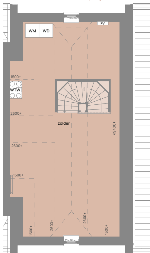
Zolderverdieping
